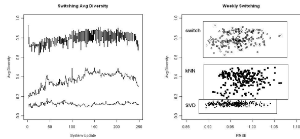
(a) Switching Temporal Diversity (b) Switching RMSE vs Diversity
