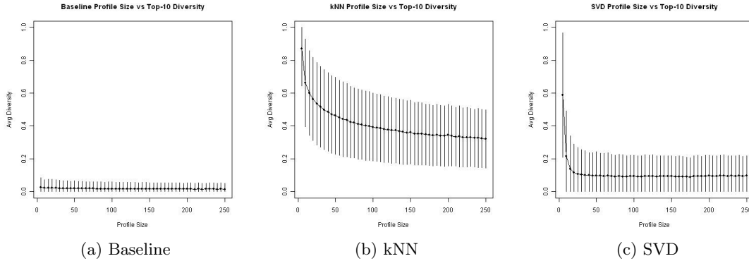
Figure 4: Profile Size vs. Top-10 Temporal Diversity for Baseline, kNN and SVD CF
