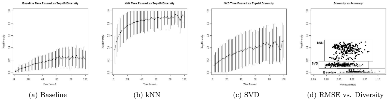
Figure 6: Time Passed vs. Top-10 Temporal Diversity for Baseline, kNN and SVD CF and Comparing Accuracy with Diversity
