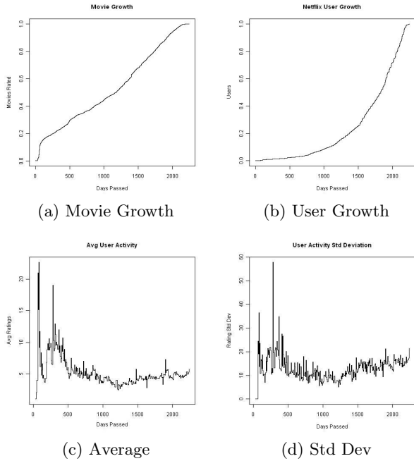
Figure 1: Growth of Netflix Dataset Over Time & Average/Standard Deviation of Returning Users’ Ratings Input Per Week
