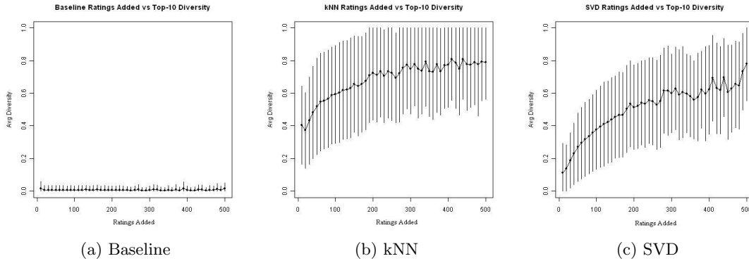
Figure 5: Ratings Added vs. Top-10 Temporal Diversity for Baseline, kNN and SVD CF
