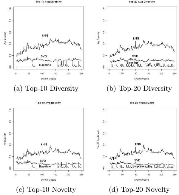
Figure 3: Top-10 and 20 Temporal Diversity and Novelty for Baseline, kNN and SVD CF
