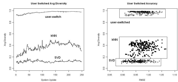
(a) Temporal Diversity (b) RMSE vs. Diversity
